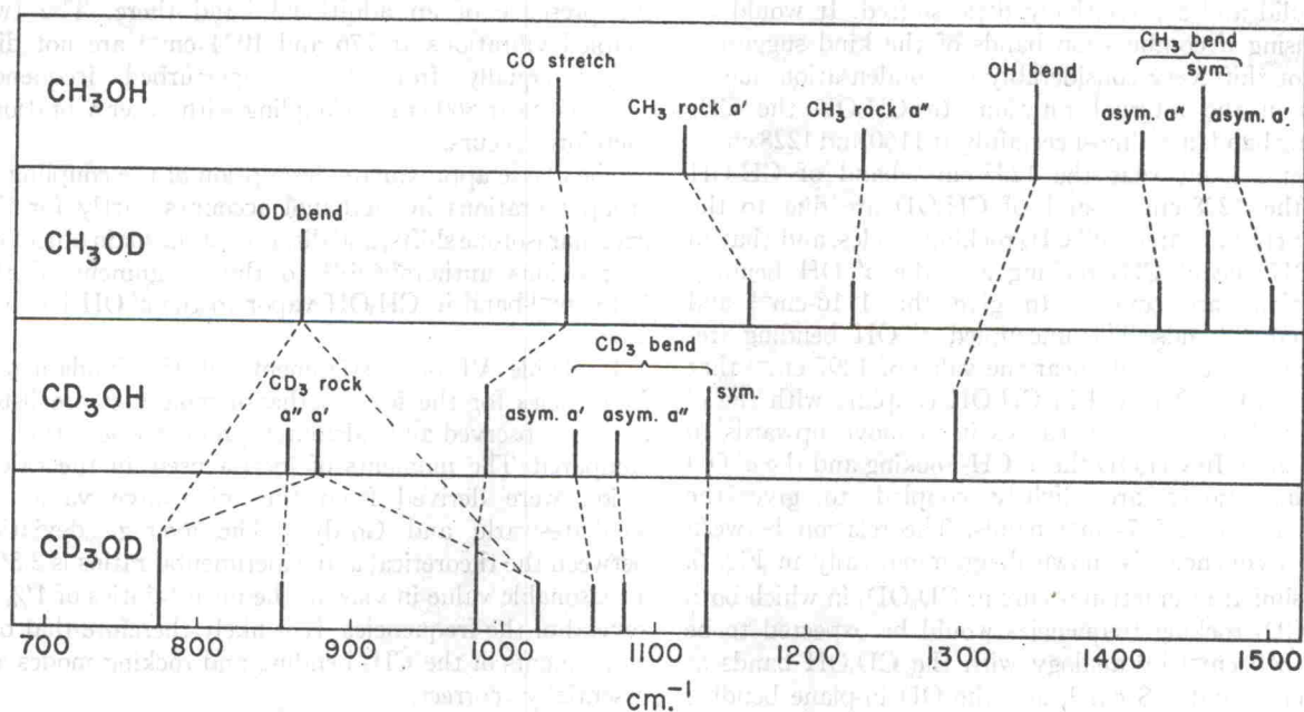
FIG. 6. Vapor-phase fundamental frequencies of the four isotopic methanols in the 700-to-1500- \text{cm}^{-1} region. Strong coupling occurs between OH bending and a' CH 3 rocking in \text{CH}_3\text{OH} ; between OD bending and a' CD 3 rocking in \text{CD}_3\text{OD} ; and between CO stretching and CD 3 symmetrical bending in \text{CD}_3\text{OH} and \text{CD}_3\text{OD} . There is also some coupling between OD bending and a' CH 3 rocking in \text{CH}_3\text{OD} .
